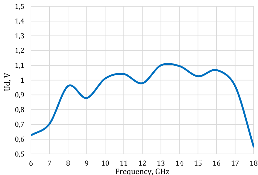
Typical power detector level vs. frequency @ P_{out} = 33 dBm
