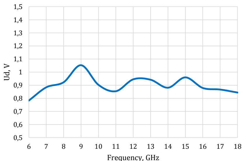
Typical power detector level vs. frequency @ P_{out} = 37 dBm
