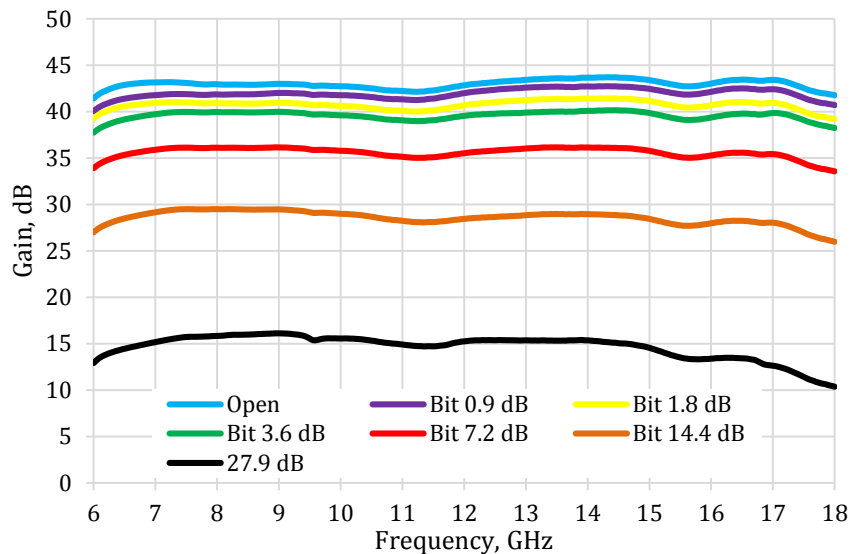
Typical small signal gain (turn on the attenuator bits)
