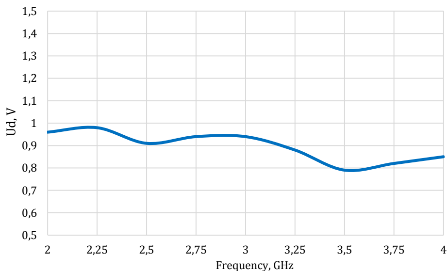
Typical power detector level vs. frequency @ P_{out} = 46 dBm
